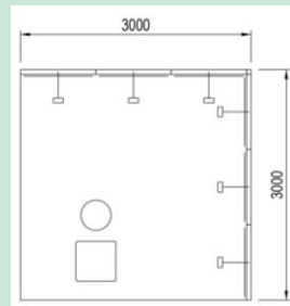
Fresh 9 m 2 (Art. 100735) 3 m x 3 m
